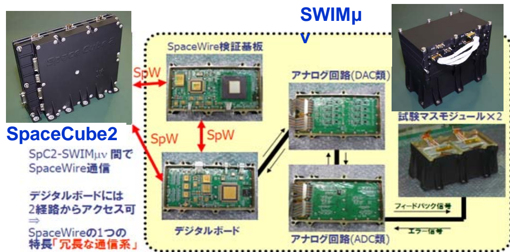
SWIMの構成(SpaceCube2とSWIM \mu v)
